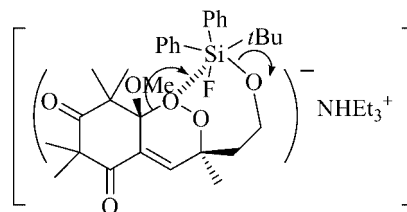
Figure 3. Proposal for a transient hexacoordinate fluorosilicon complex.
