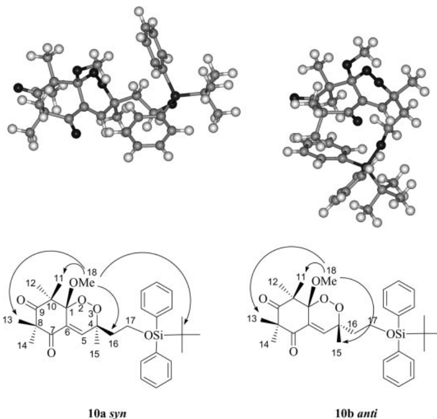
Figure 2. Modelling and NOESY experiments for 10a and 10b endoperoxides.
