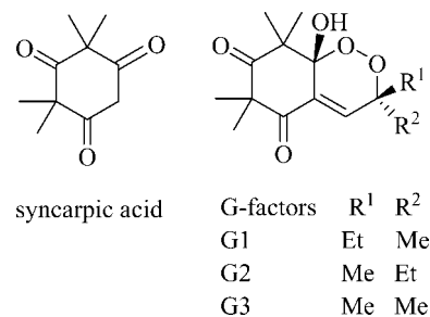
Figure 1. Syncarpic acid, G-factors.
