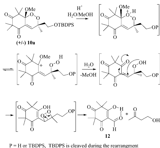
Scheme 4. Acidic fragmentation of the syn endoperoxide 10a through formation of a 1,2-dioxetane.
