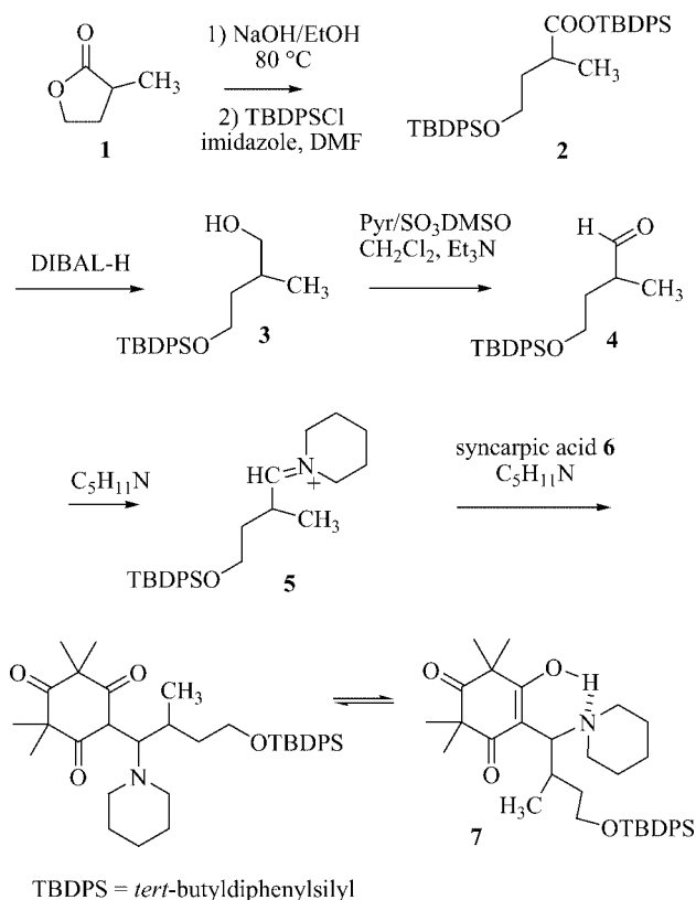
Scheme 2. Synthesis of Mannich base 7 .
