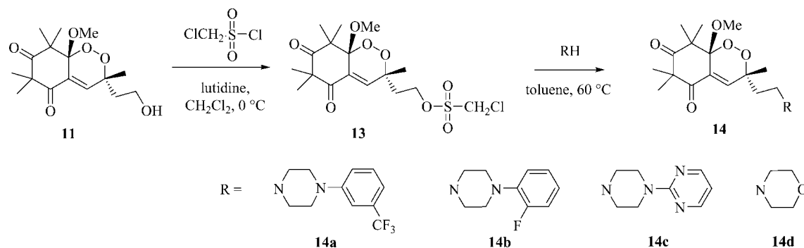
Scheme 5. Synthesis of 14a , 14b , 14c and 14d endoperoxides via monochlate 13 .
