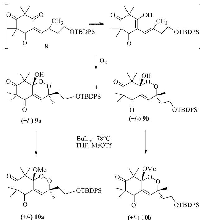
Scheme 3. Preparation of the diastereoisomeric protected endoperoxides 10a and 10b .
