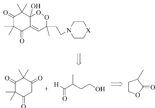
Scheme 1. Retrosynthetic approach.
